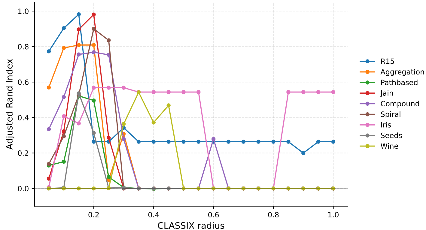
CLASSIX: ARI vs. radius (minPts=5)
