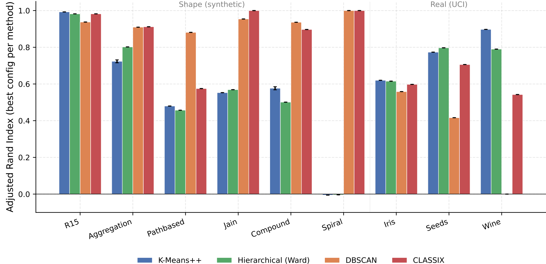
Best clustering quality per dataset across four methods
