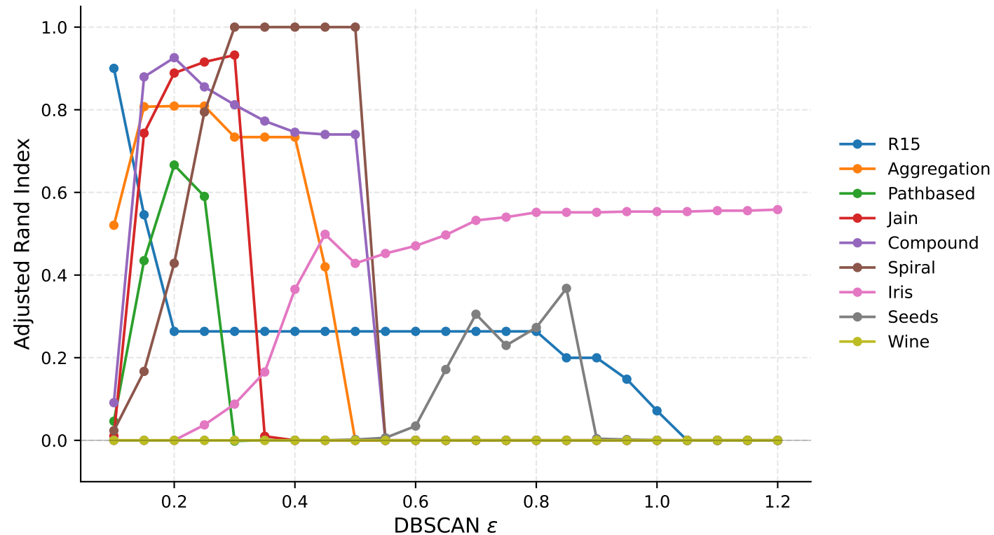
DBSCAN: ARI vs. \varepsilon (min_samples=5)
