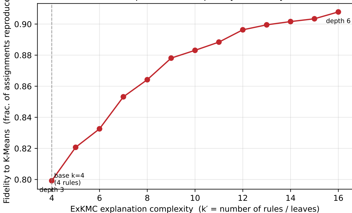
Ch5 trade-off: explanation complexity vs fidelity (UCI RFM)
