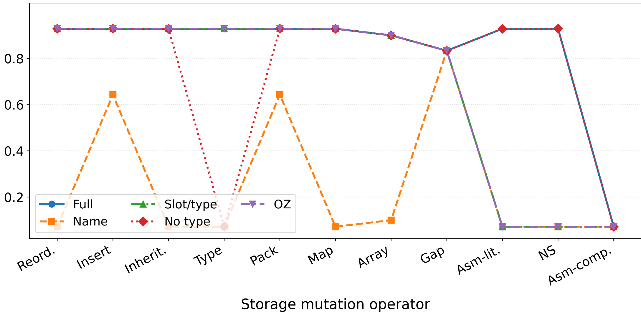
Detection estimate
