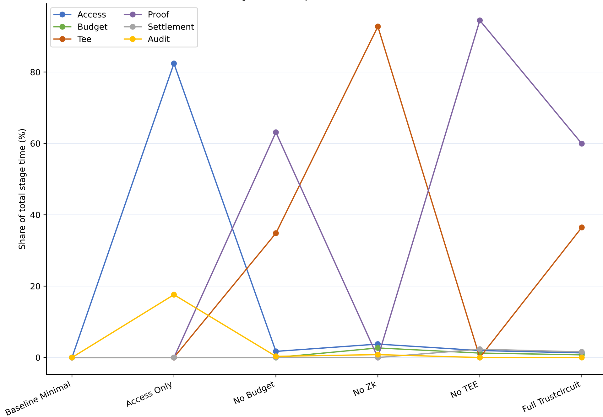
Stage-time composition across ablations
