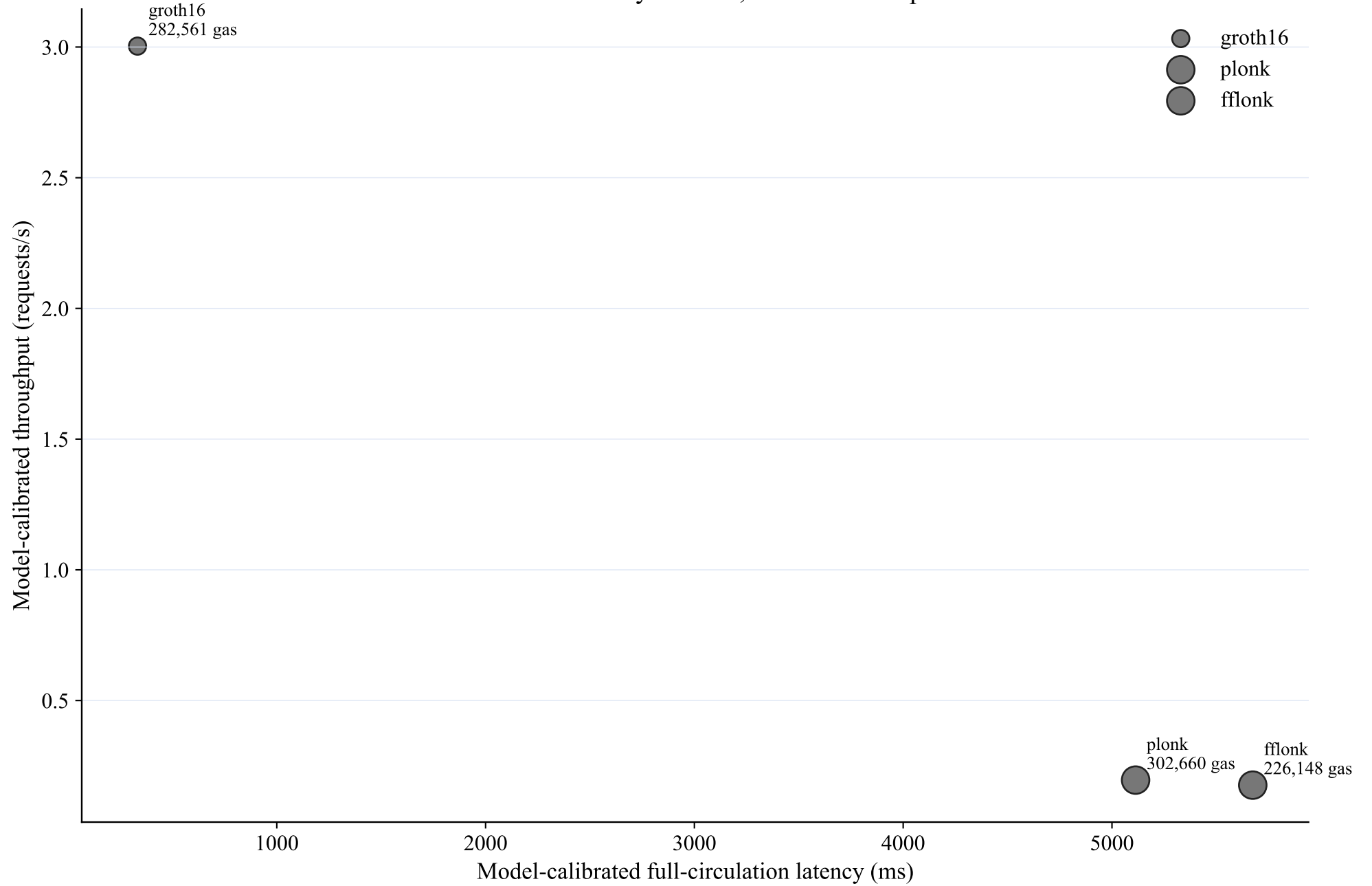
Proof-backend efficiency frontier; bubble area = proof size
