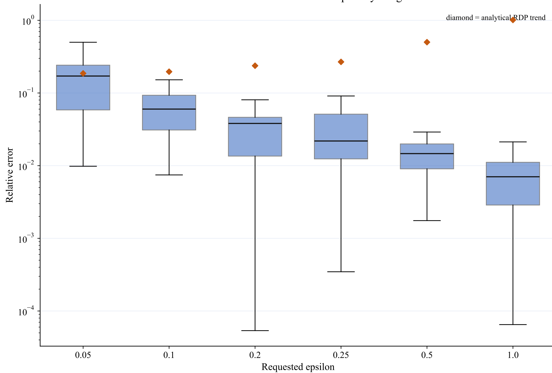
Relative-error distributions across privacy budgets
