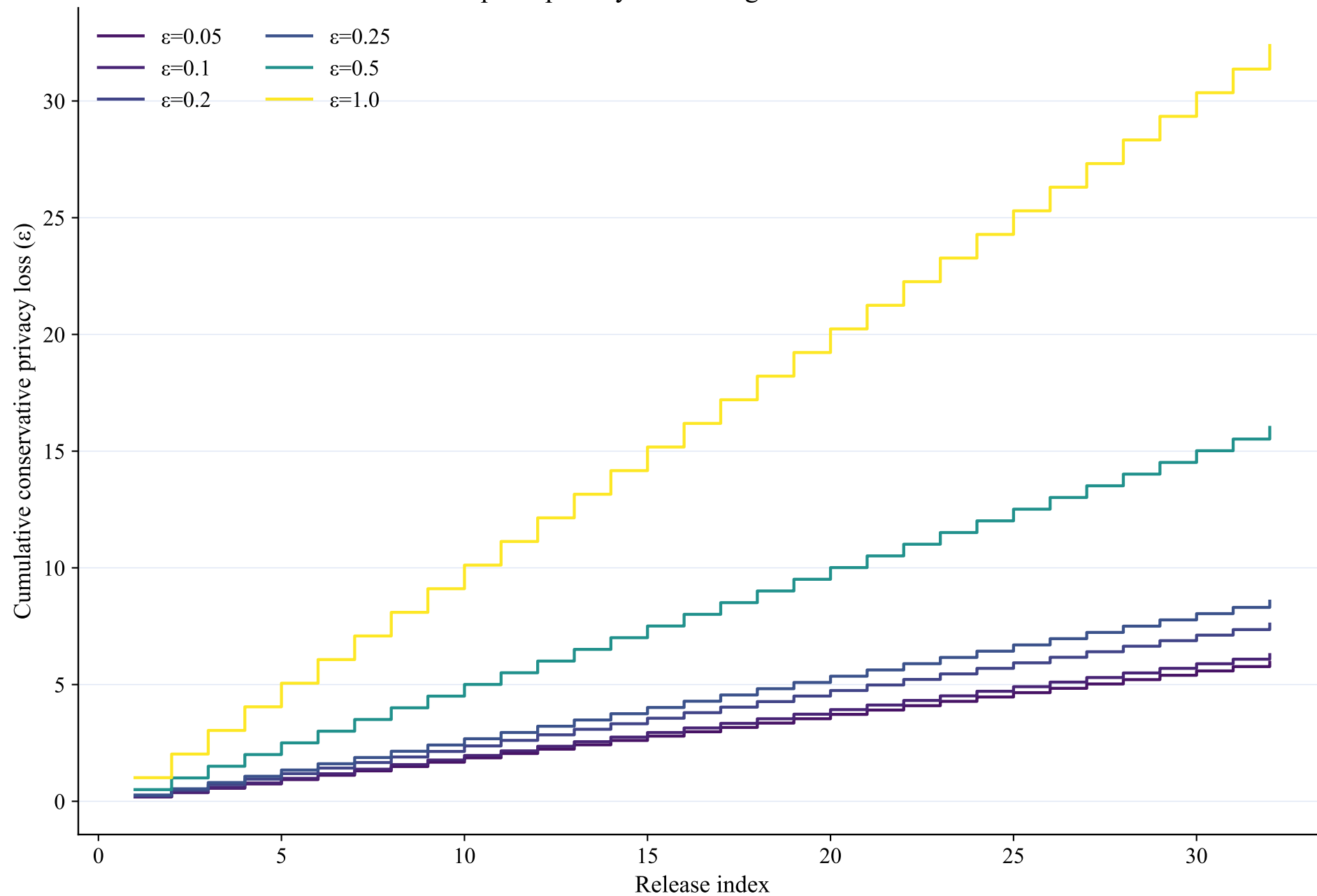
Fixed-point privacy accounting as a release staircase
