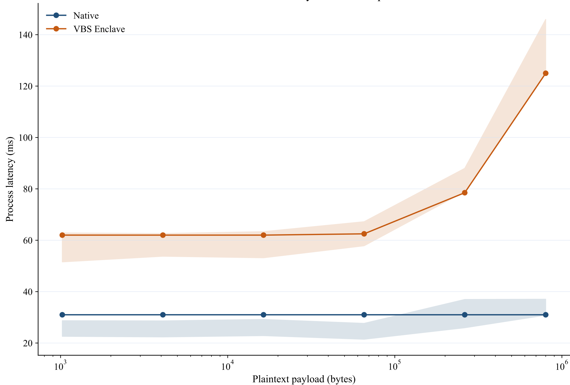
Native and VBS Enclave latency with bootstrap 95% intervals
