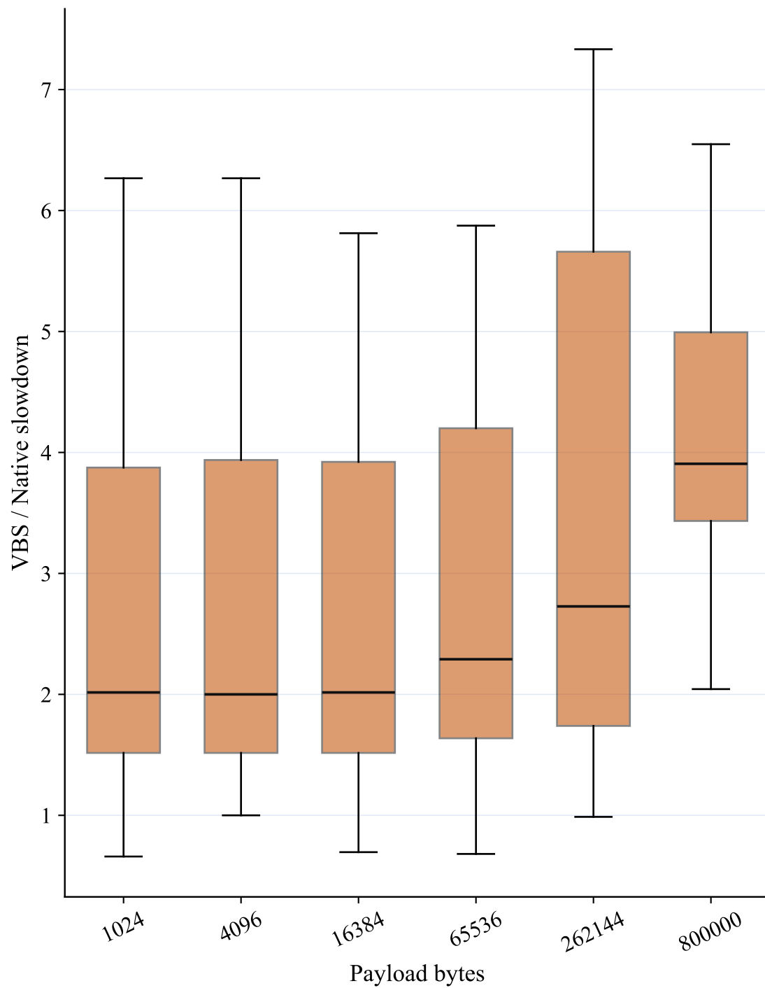
VBS overhead distributions and incremental CPU cost
