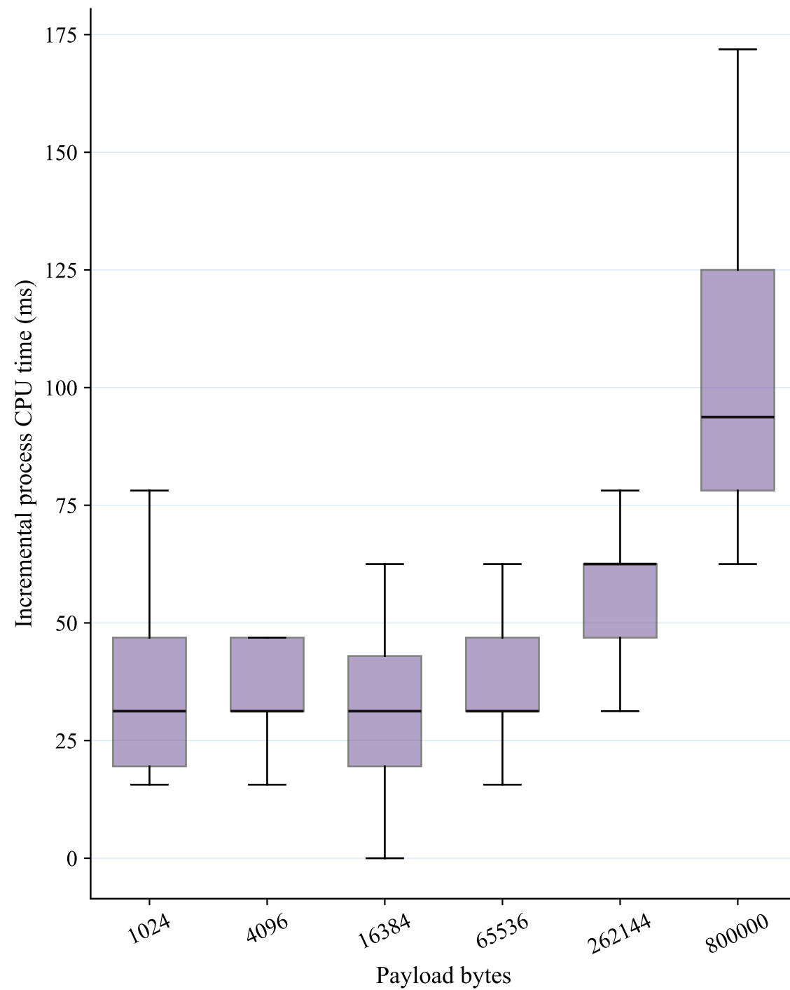
VBS overhead distributions and incremental CPU cost
