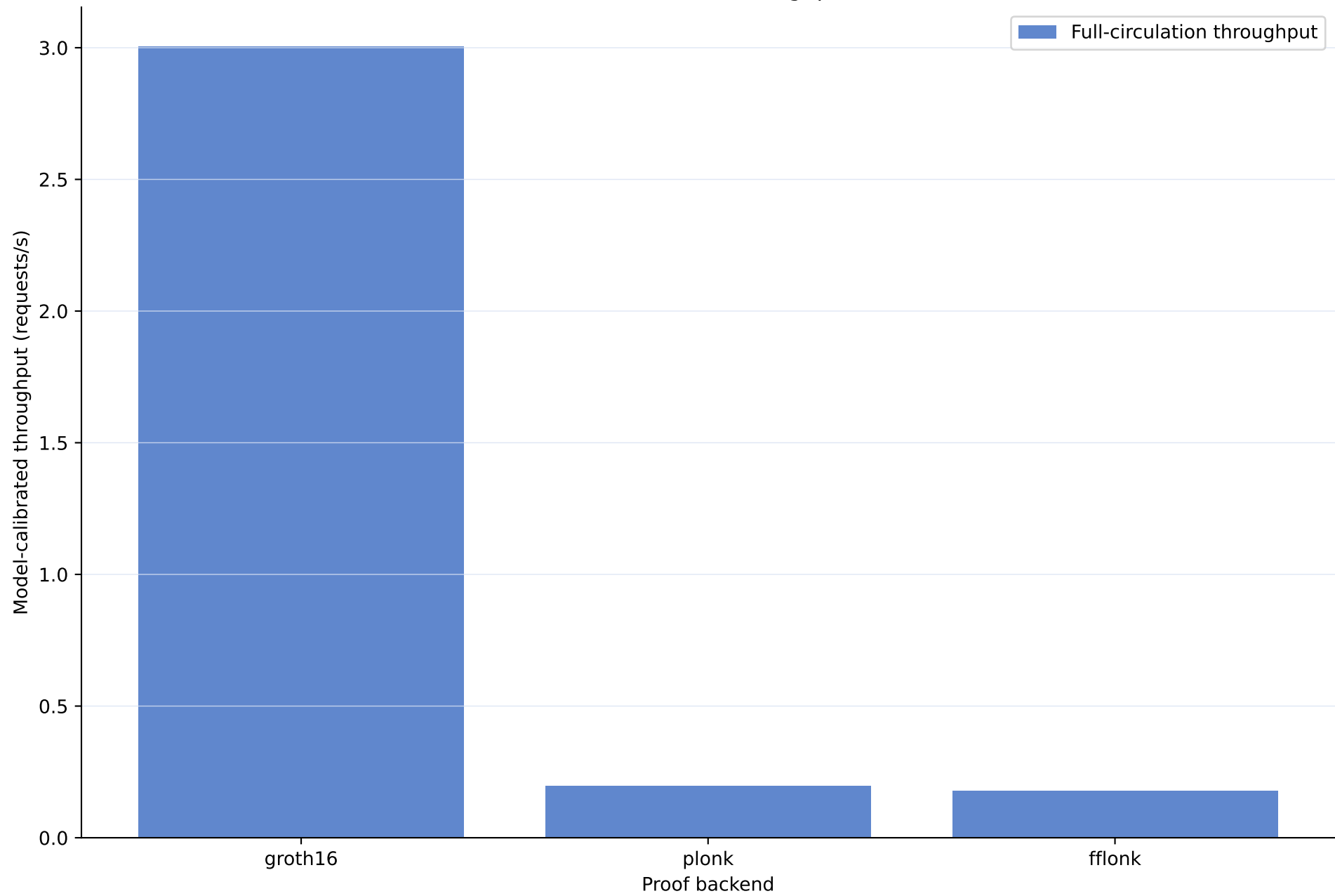
Proof-backend throughput
