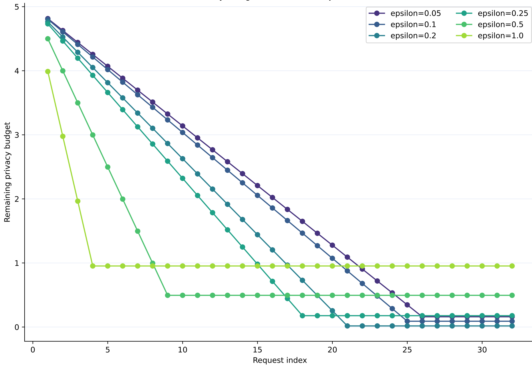
Privacy-budget exhaustion trajectories
