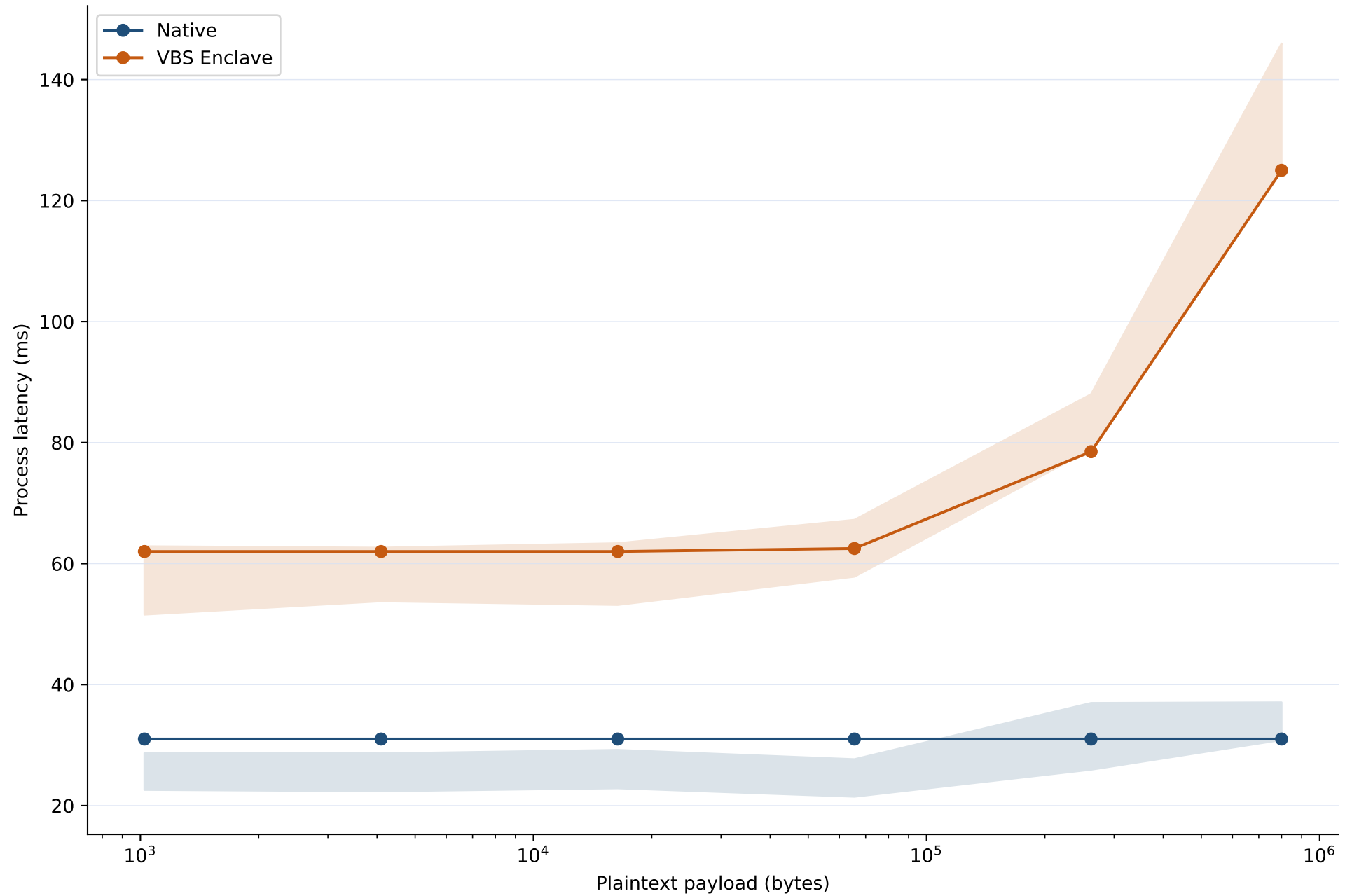
Native and VBS Enclave latency
