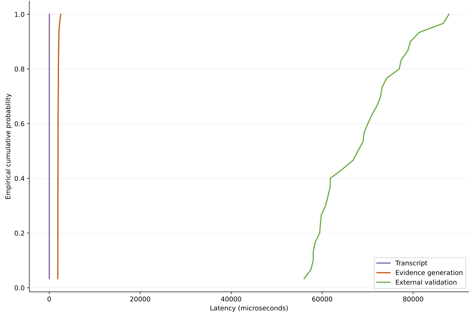
Transcript, evidence, and validation overhead
