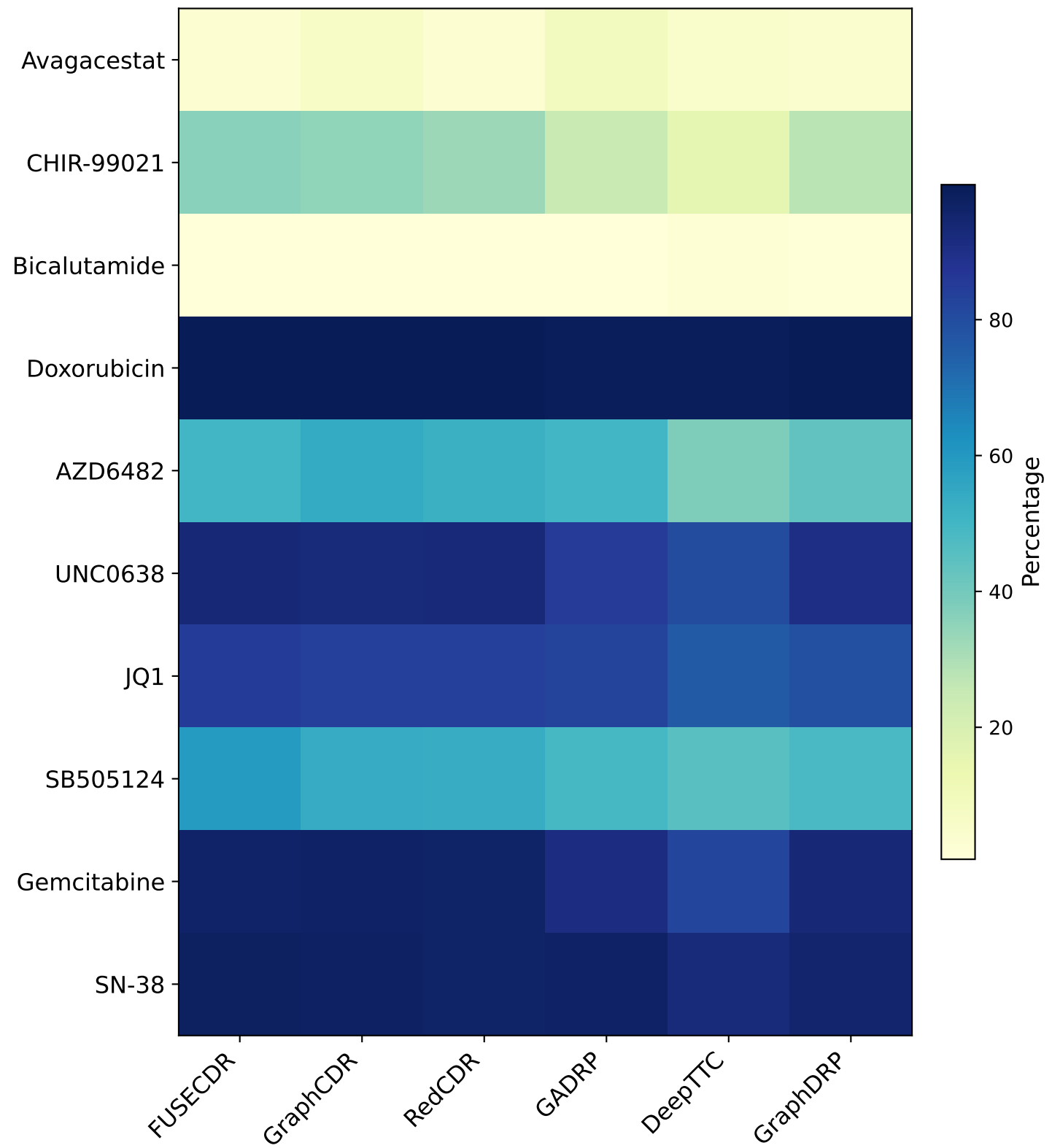
Drug-Level AUPR
