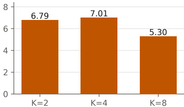
Mean would-halt ACT steps (record level)
