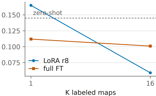
Dynamic (maze-dense, U-Net)
