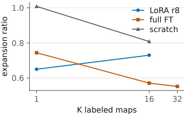
Static (maze-dense, HRM)
