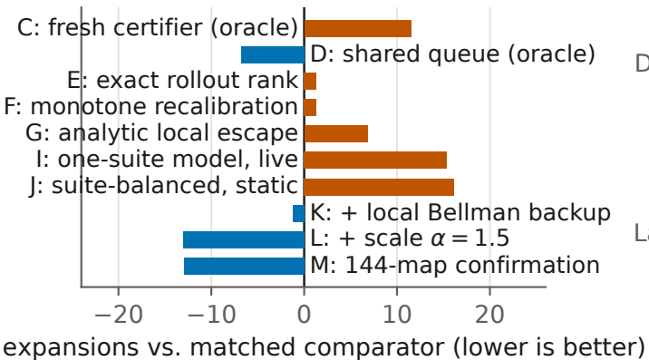
(a) Mechanism ladder
