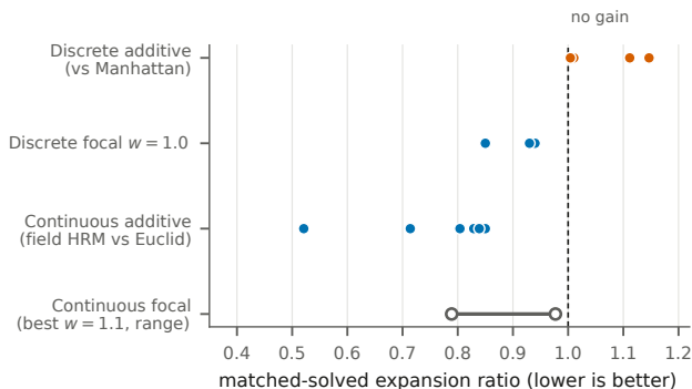
Figure 2: The integration inversion. Against a tight Manhattan baseline on discrete grids, additive learned magnitude is inert or harmful, whereas the same frozen predictions reduce expansions by 6–15% as a ranker inside the tested focal band. Against a loose Euclidean baseline on continuous hard roadmaps, additive guidance reduces matched expansions by 15–48%; focal variants recover less.
