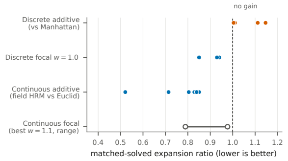
Figure 2: Integration summary across substrates (moved from the main paper). Discrete grids (Manhattan anchor): additive learned magnitude is at or below baseline while the same trained predictions reduce expansions by 6–15% as a within-band ranker at w=1.0 . Continuous roadmaps (Euclidean anchor): additive guidance reduces matched expansions by 15–48%; the plotted focal w=1.1 range is an exploratory, post-hoc operating point and is not used for any main-paper claim.
