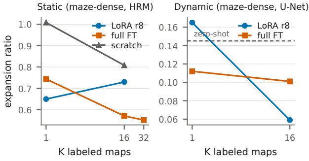
Figure 3: Illustrative K -indexed adaptation curves on the static (left) and dynamic (right) dense-maze targets (moved from the main paper; the factorial figure there supersedes them as the primary adaptation visual). On this static target, LoRA leads at K=1 and full fine-tuning overtakes it by K=16 ; on the dynamic target the low-supervision failure is not observed in the K -indexed protocol. Curves connect the evaluated K values for one backbone per panel; quoted inference is map-clustered.
