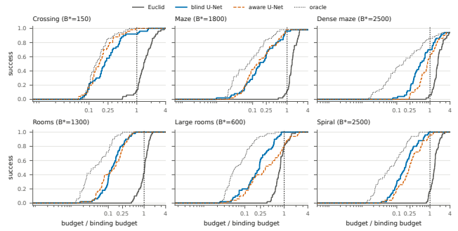
Figure 1: Success-vs-budget step curves per dynamic suite (fresh 50-map cohort), derived exactly from one 4 \times -binding evaluation pass. Budgets are normalized by the binding budget B^* (dashed vertical line). The learned providers reach high success at 0.05\text{--}0.3 \times B^* ; Euclid requires 1.7\text{--}2.8 \times B^* to match the blind provider’s binding-budget success.
