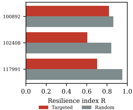
(c) R after removing 10% of nodes
