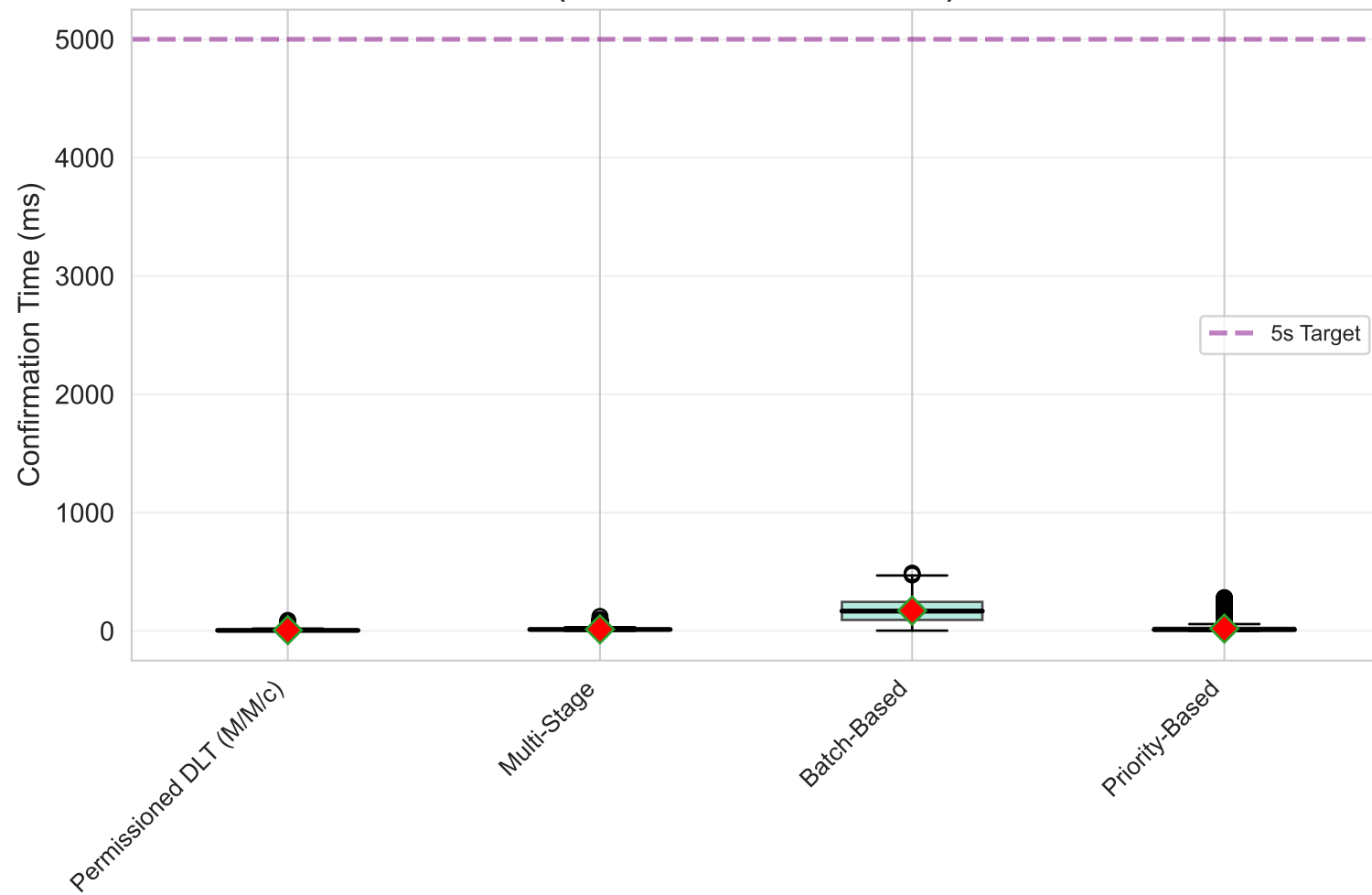
Box Plot Comparison (Viable Models at 200 TPS)
