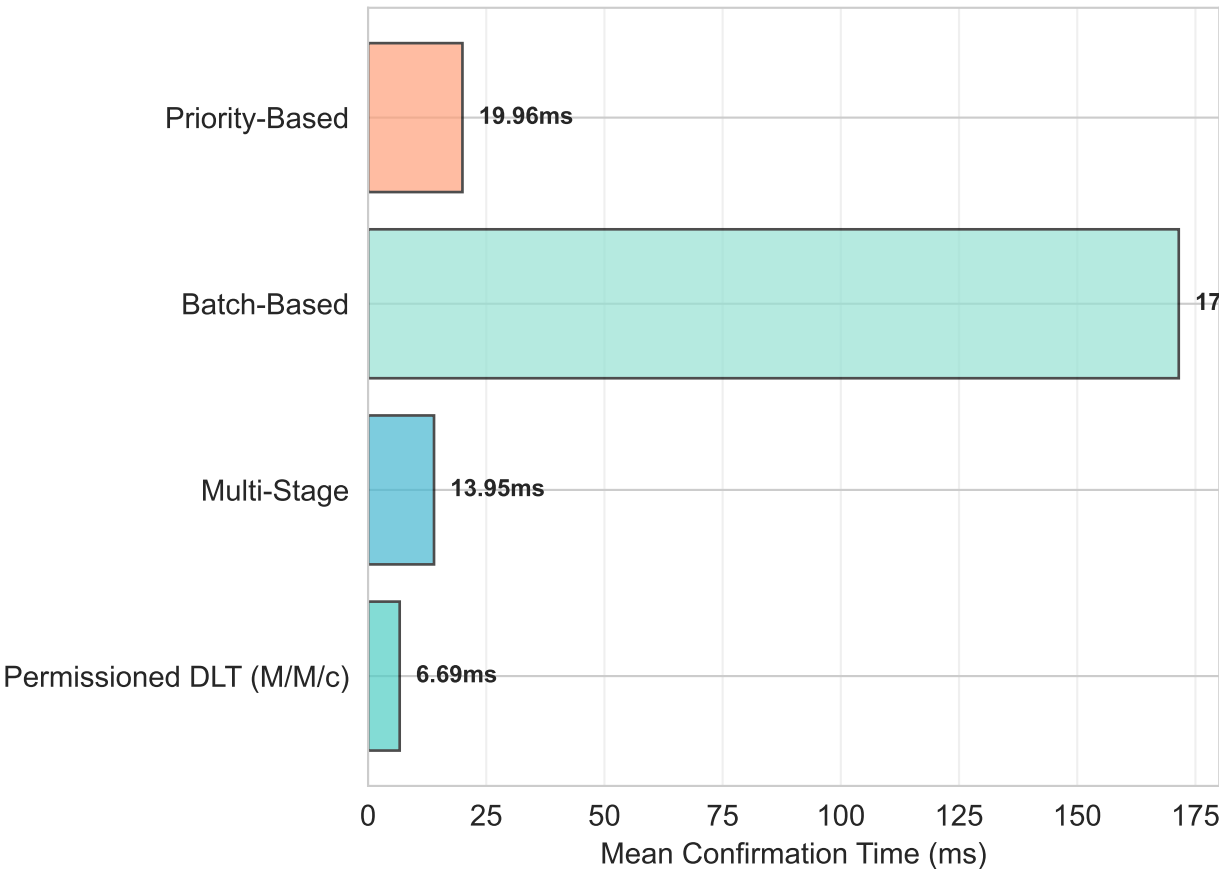
Mean Confirmation Time Comparison (Stable Models at 200 TPS)
