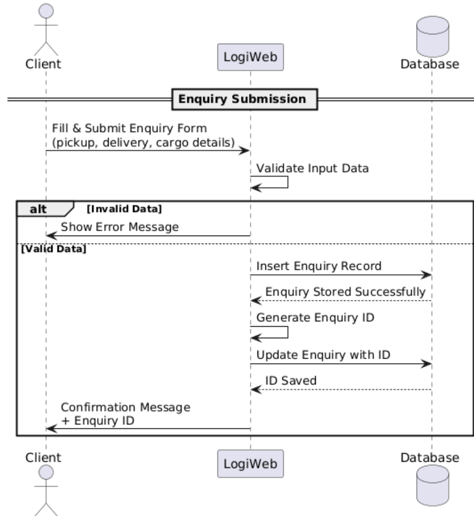
ENQUIRY_SUBMISSION_SEQUENCE_DIAGRAM
