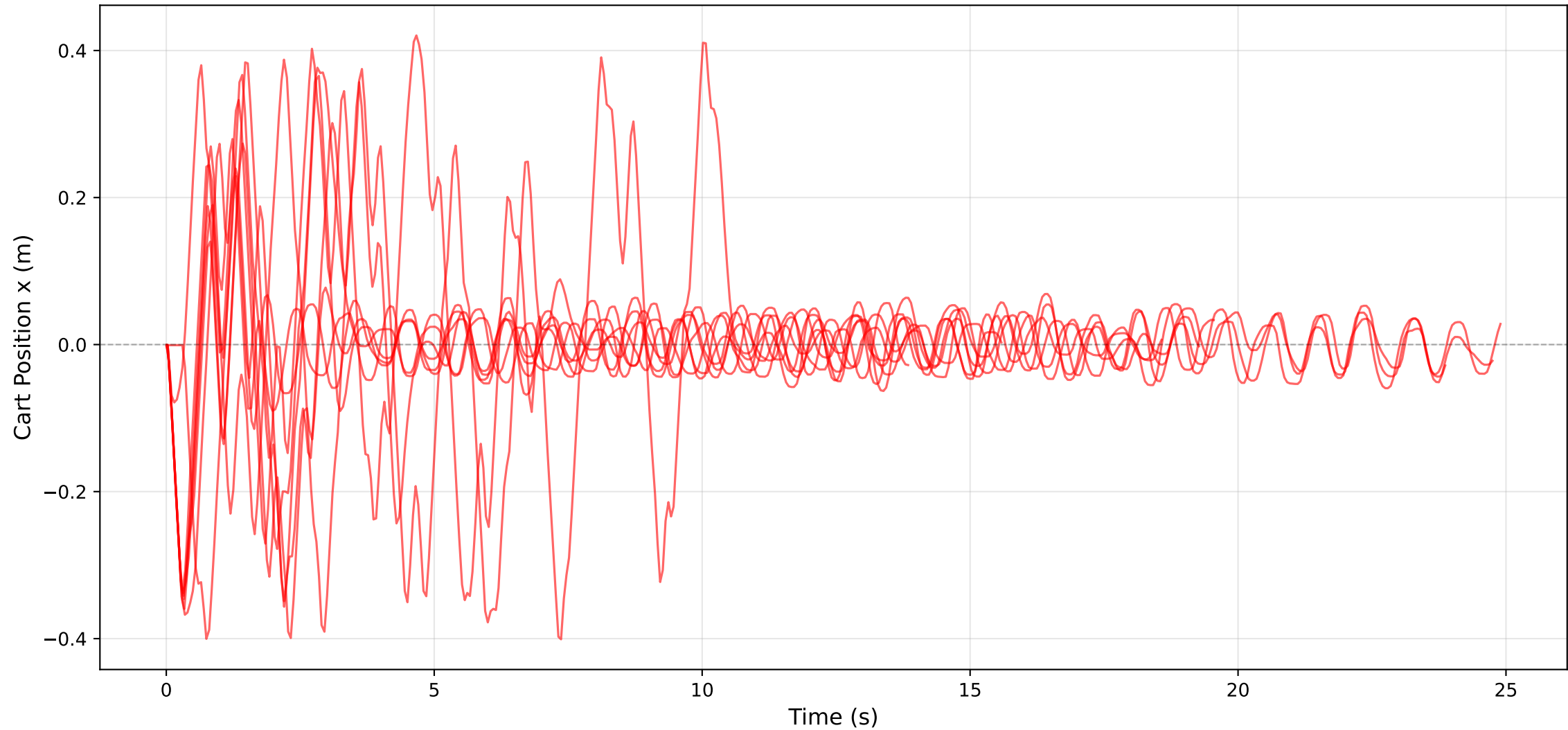
MPC Trajectories (8 runs)
