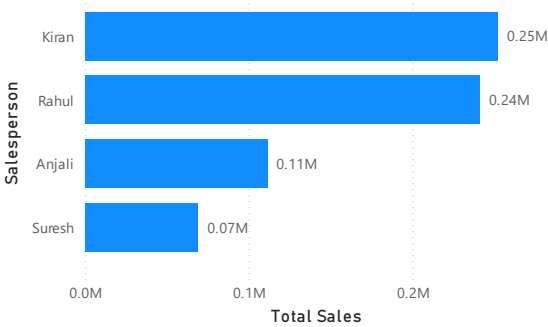
Sales by Salesperson
