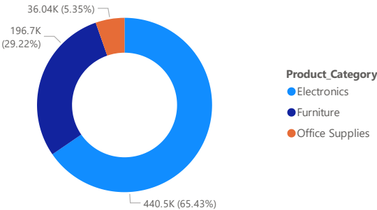
Sales by Product Category
