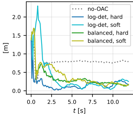
Follower-position error
