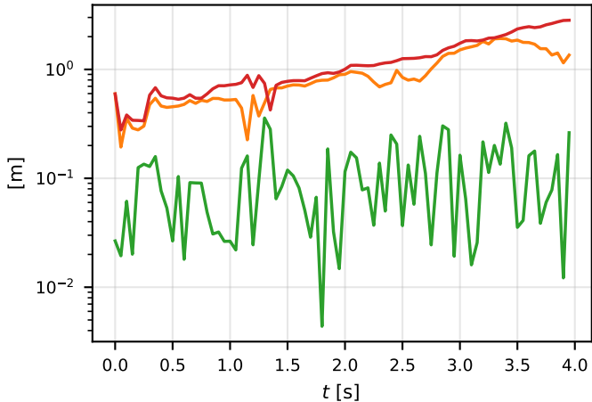
Follower-position error
