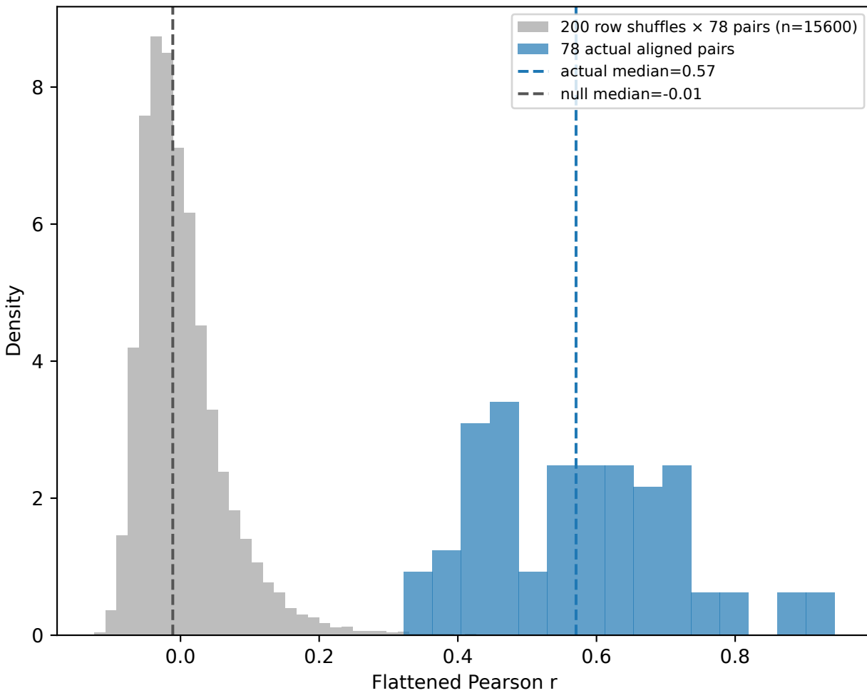
Actual fixed-channel alignment versus row-shuffle null
