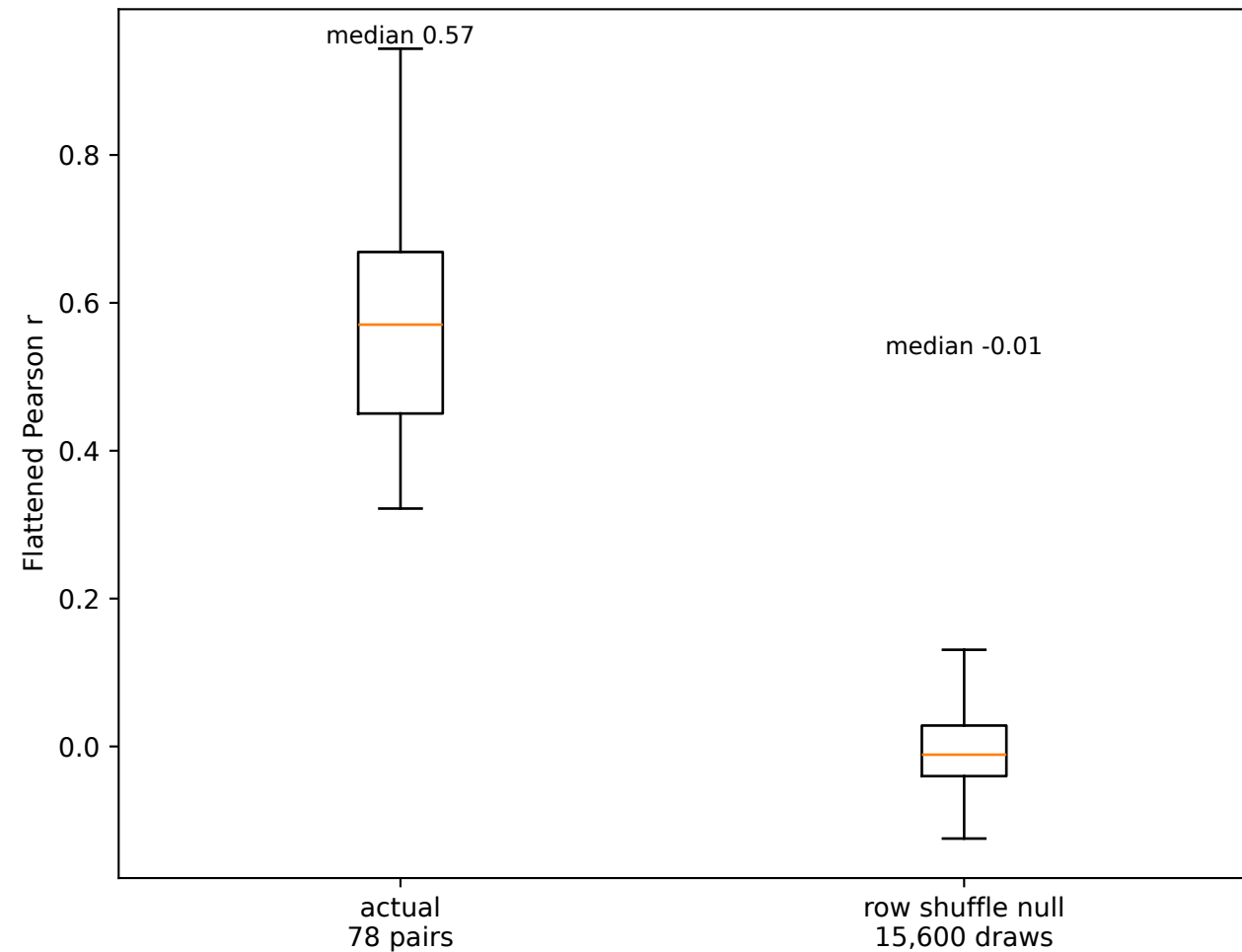
Distribution comparison; no independent-pair p-value
