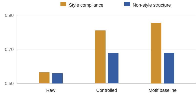
(b) Score decomposition
