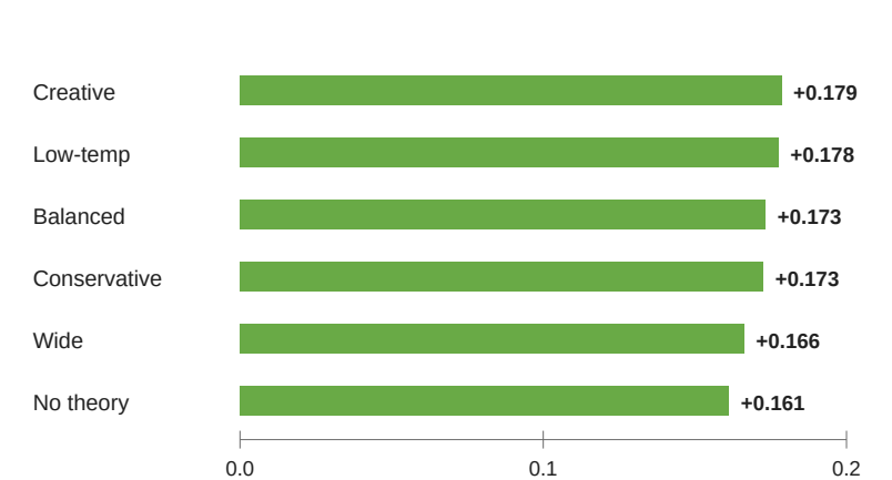
(c) Controlled minus raw by preset
