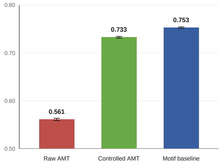
(a) Composite score with 95% CI
