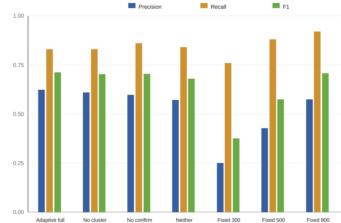
(a) Boundary precision, recall, and F1
