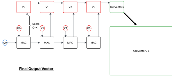
(a) Single-row dataflow. Query Q_0 streams left-to-right through MAC columns; each column computes score s_i = Q_0 \cdot K_i and feeds the stationary V_i register above. After the final column, OutVectors accumulates the weighted sum and normalises by l_N to produce OutVector / L .
