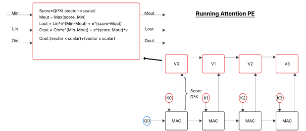
(b) Running Attention PE detail. The PE receives running state (M_{in}, L_{in}, O_{in}) and score s_i = Q_i \cdot K_i (computed below by the MAC array), then updates: M_{out} = \max(M_{in}, s_i) ; L_{out} = L_{in} e^{M_{in} - M_{out}} + e^{s_i - M_{out}} ; O_{out} = O_{in} e^{M_{in} - M_{out}} + e^{s_i - M_{out}} \cdot V_i . Updated state (M_{out}, L_{out}, O_{out}) passes right.
