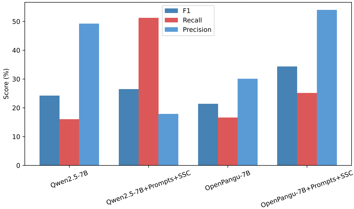
Goal Interpretation: All Metrics Comparison
