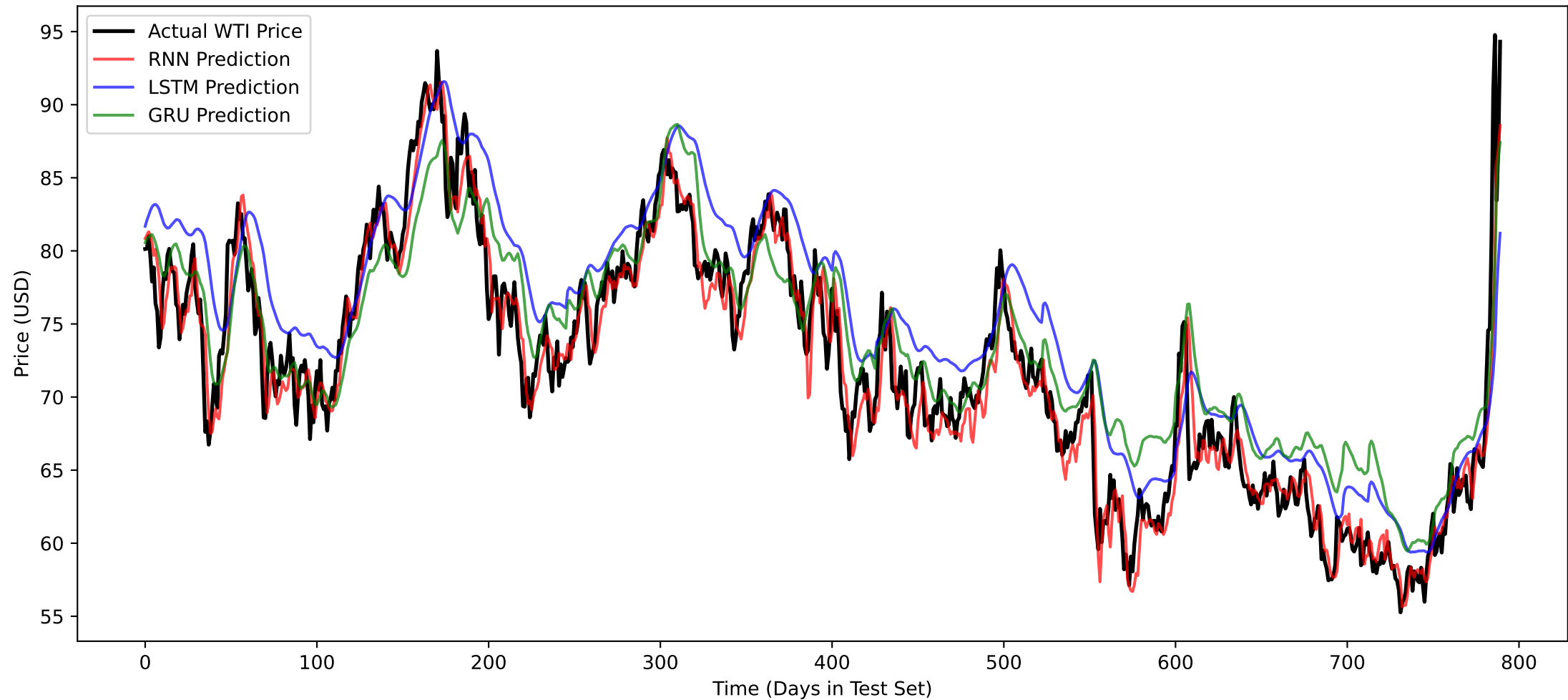
WTI Crude Oil Price: Actual vs Predicted
