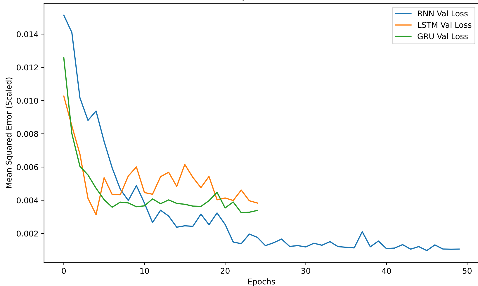
Validation Loss Comparison Across Architectures
