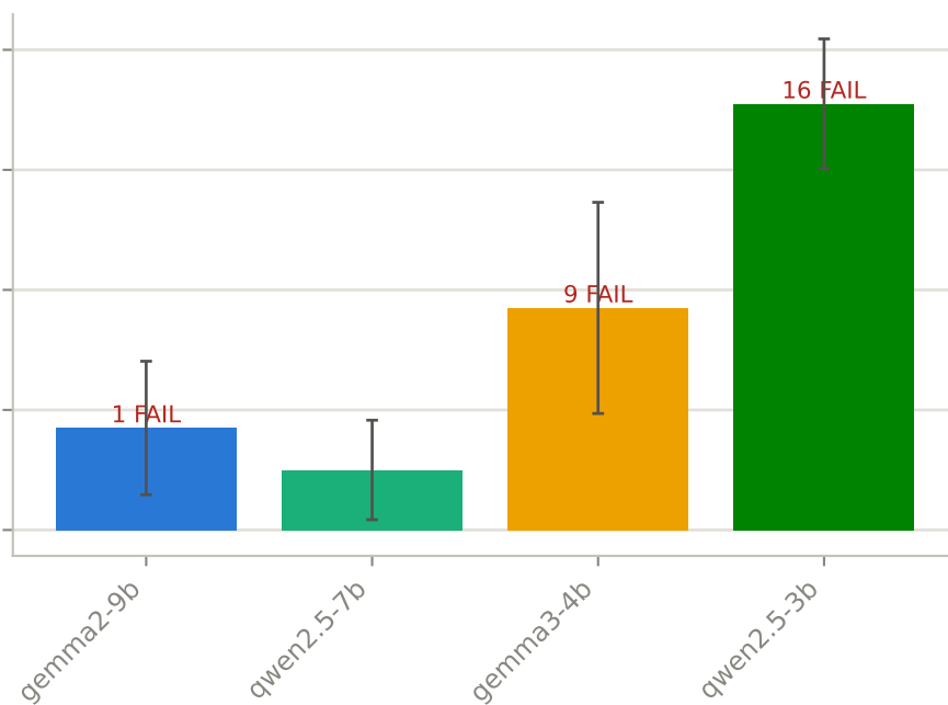
schema-based
