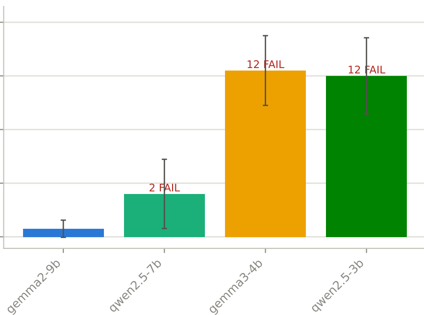
zero-shot
