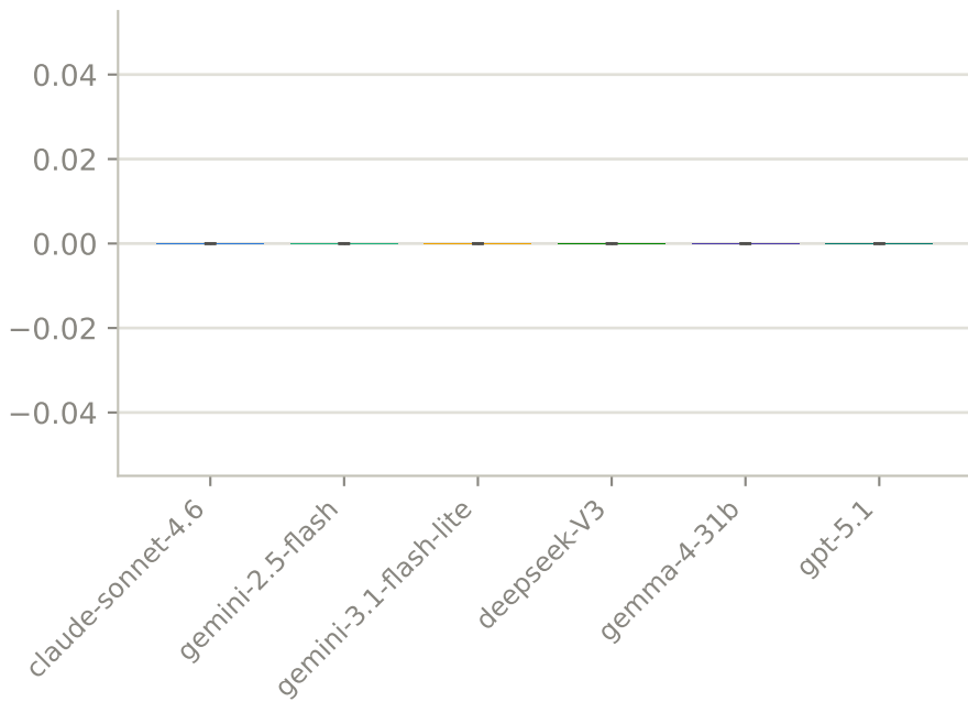
zero-shot
