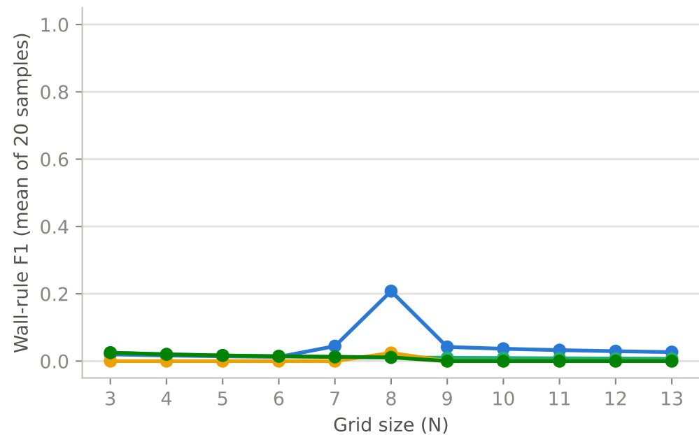
zero-shot
