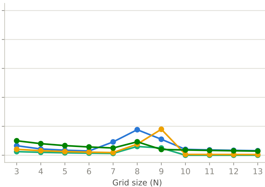
schema-based
