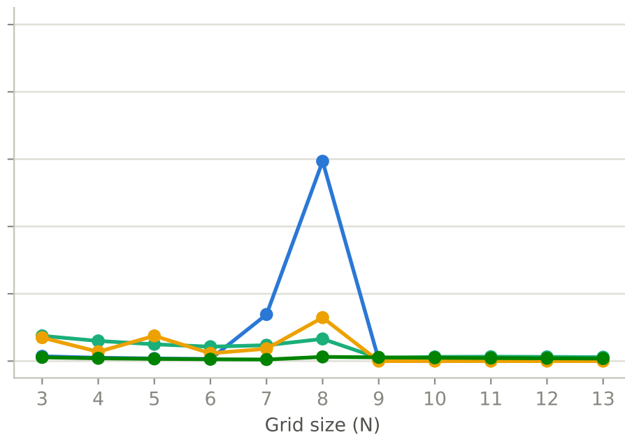
one-shot
