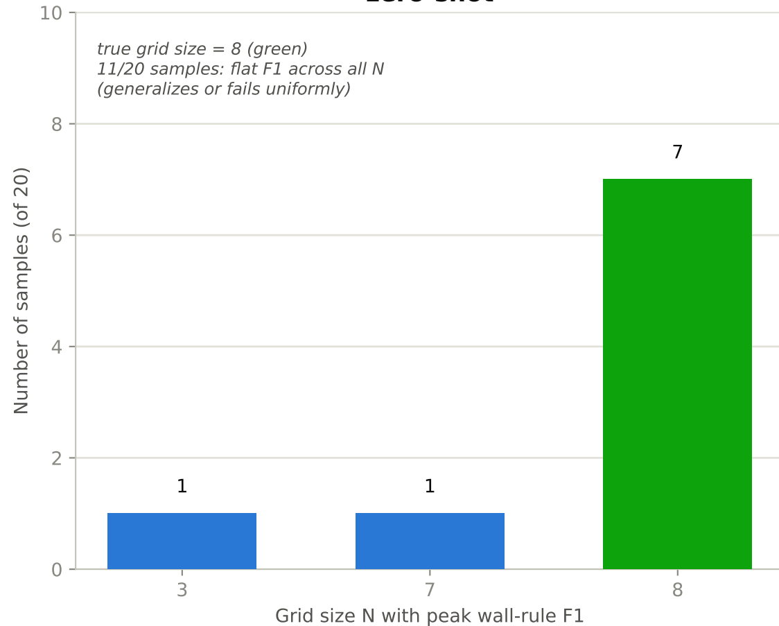
zero-shot
