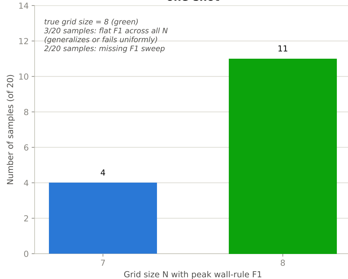
one-shot
