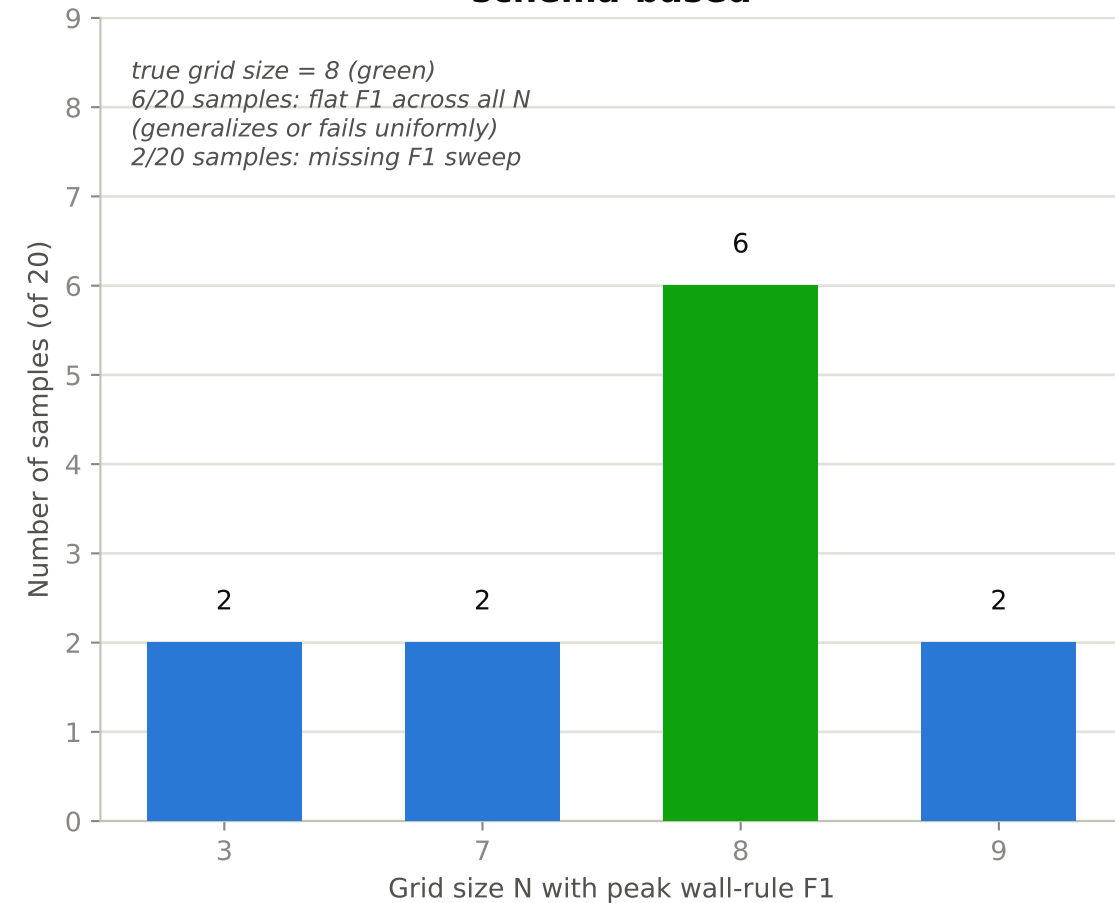
schema-based
