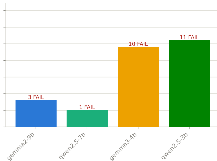
one-shot
