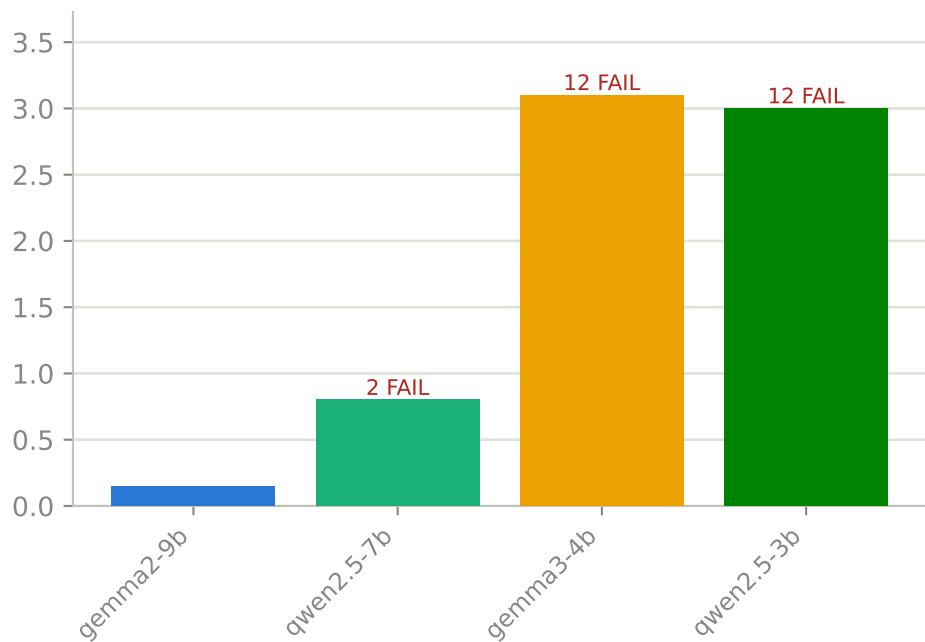
zero-shot
