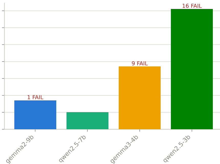
schema-based
