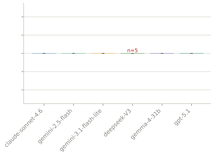
one-shot
