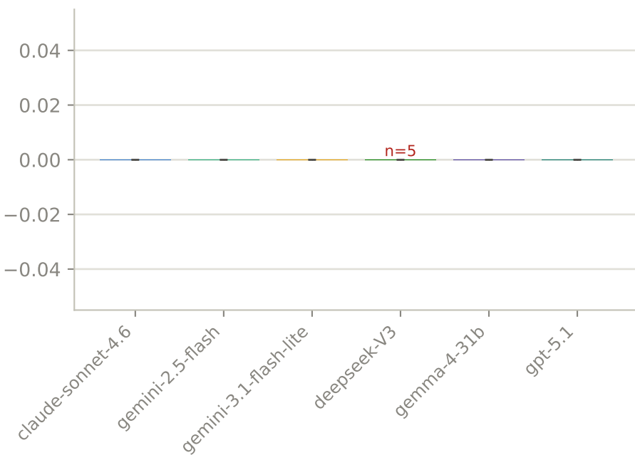
zero-shot
