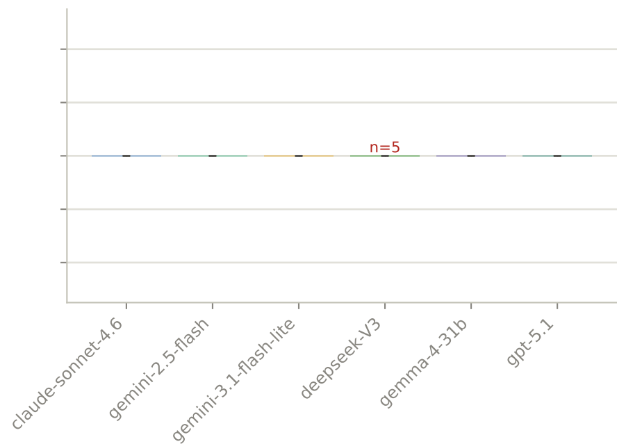
schema-based
