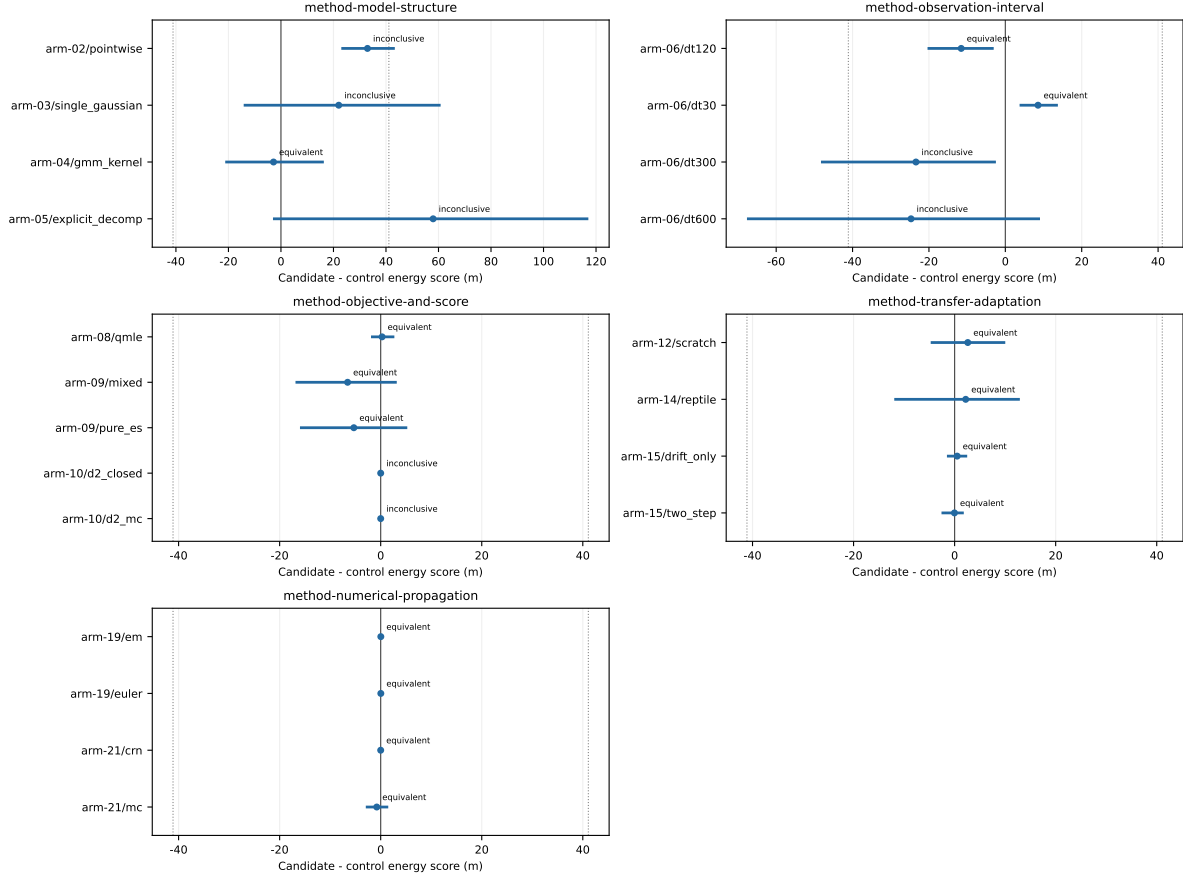
Figure 1: Actual audit-bound primary method comparison plot. Intervals and the fixed practical band are retained from the original analysis. Displayed verdicts are finite-algorithm recorded states, not resolution-invariant qualification or accepted scientific claims.
