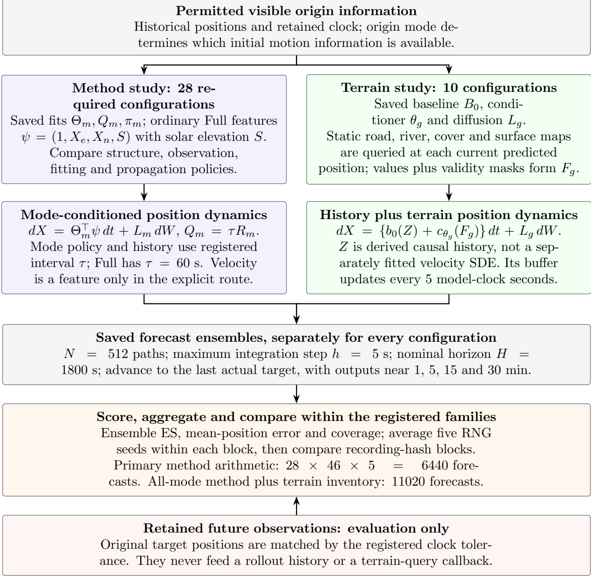
Figure 10: Executed-model and evaluation data flow, not an additional experiment or a neural architecture. The two branches have independent fitted models and controls. The future-observation arrow ends at scoring, not prediction. \tau (observation/history interval), h (integration step) and H (forecast duration) are distinct; N and five RNG seeds are simulation resources, not independent observed people. The nominal time axis is conditional on retained clock provenance.
