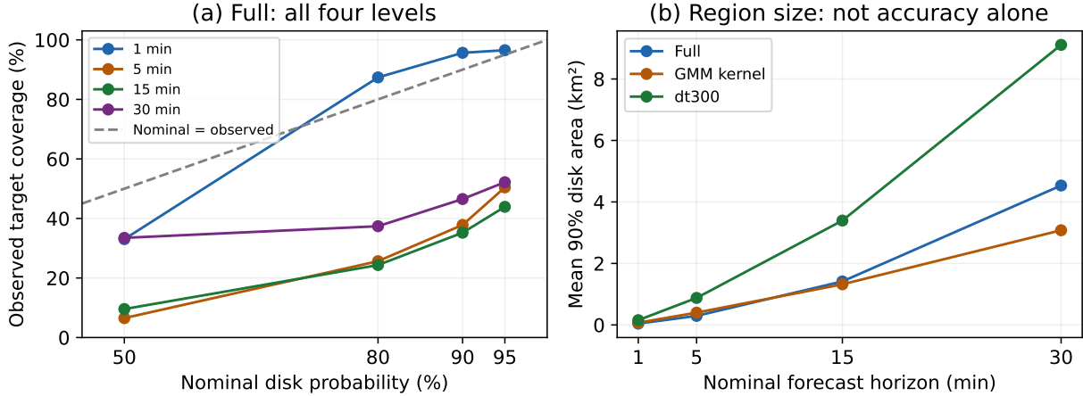
Figure 15: Saved calibration and region-size diagnostics, not new experiments. Left: Full’s observed coverage against nominal probability, separately for each horizon; the diagonal denotes nominal agreement. Right: mean 90% disk area for the three previously displayed models. Connecting lines only guide the eye between four measured levels or horizons; there is no intermediate target evaluation, simultaneous path coverage, or new statistical test.
