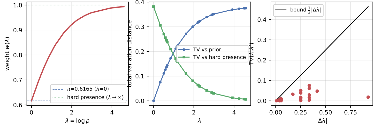
(a) soft-evidence weight (logistic) (b) soft evidence interpolates prior <math>\pi=0.6165</math> (c) hard TV-Lipschitz: max TV/| \leq \frac{1}{2}
