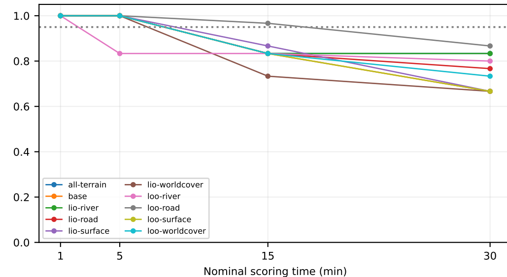
95% region coverage (probability)
