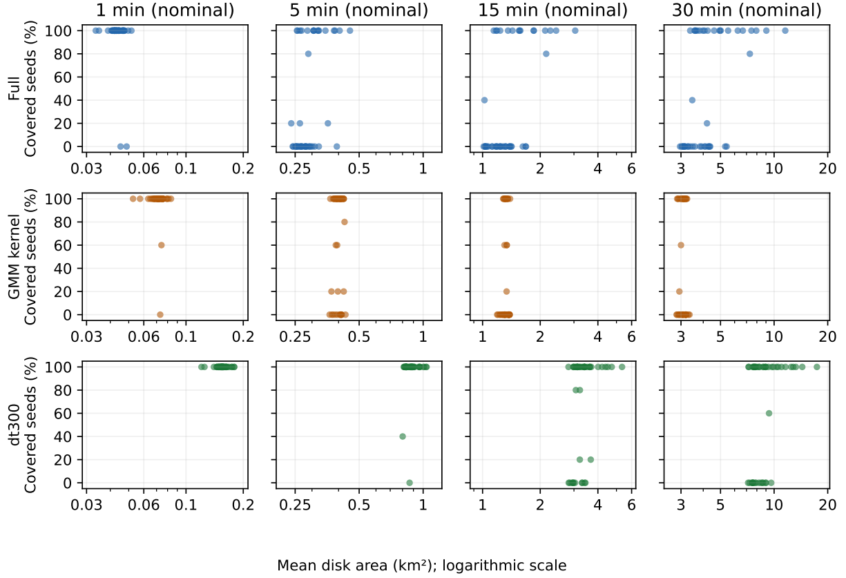
Figure 7: Paired block-level size and containment for the three previously displayed models at four nominal horizons. Each point is one recording block averaged over five forecast seeds; points can overlap. Area uses a logarithmic scale, shared across models within each horizon, while containment is the fraction of five saved disks containing the same target. These are not 46 estimates of population calibration; no simultaneous path coverage, new hypothesis test or post-hoc radius rescaling is performed.
