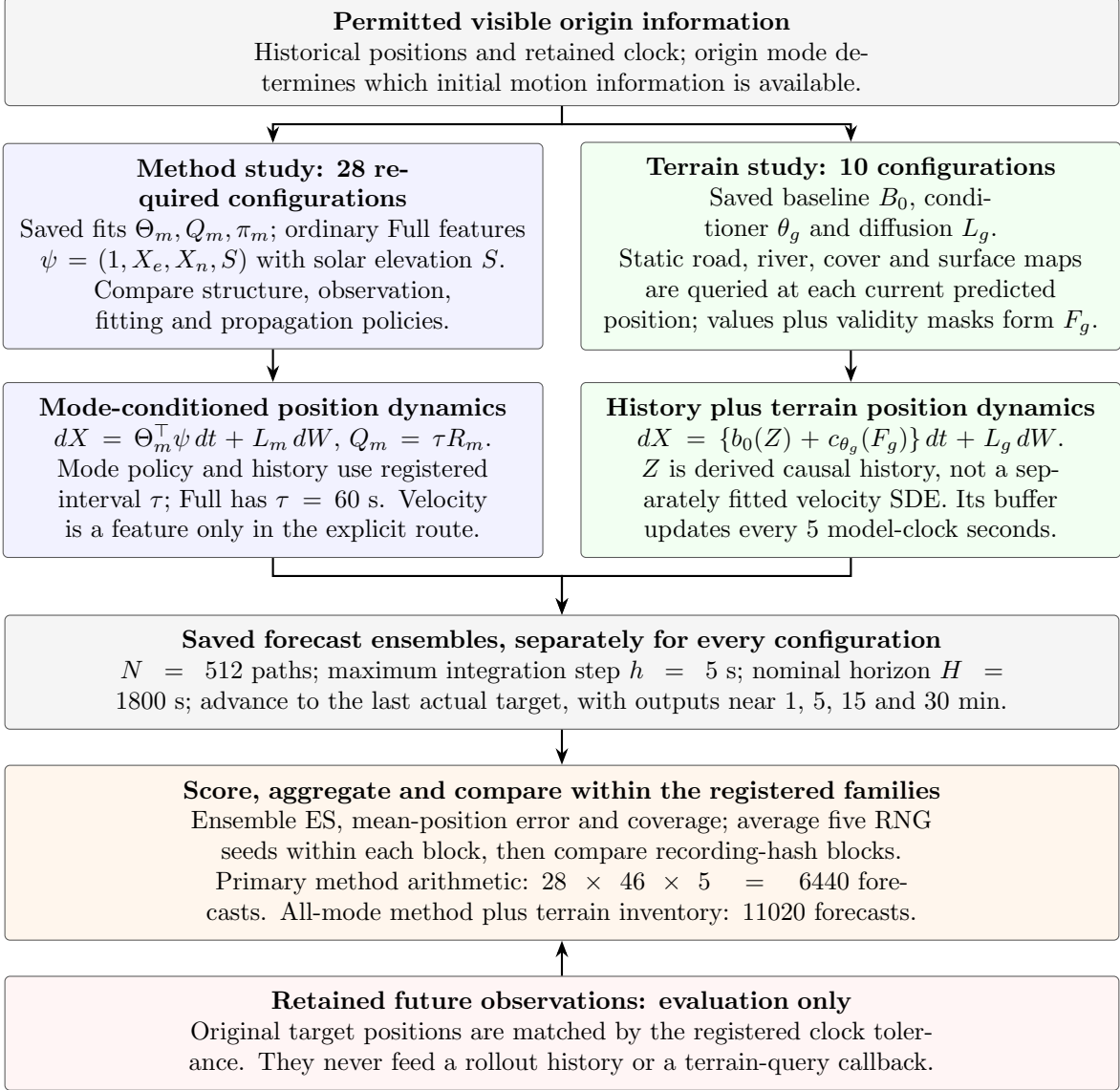
Figure 1: Executed-model and evaluation data flow, not an additional experiment or a neural architecture. The two branches have independent fitted models and controls. The future-observation arrow ends at scoring, not prediction. \tau (observation/history interval), h (integration step) and H (forecast duration) are distinct; N and five RNG seeds are simulation resources, not independent observed people. The nominal time axis is conditional on retained clock provenance.
