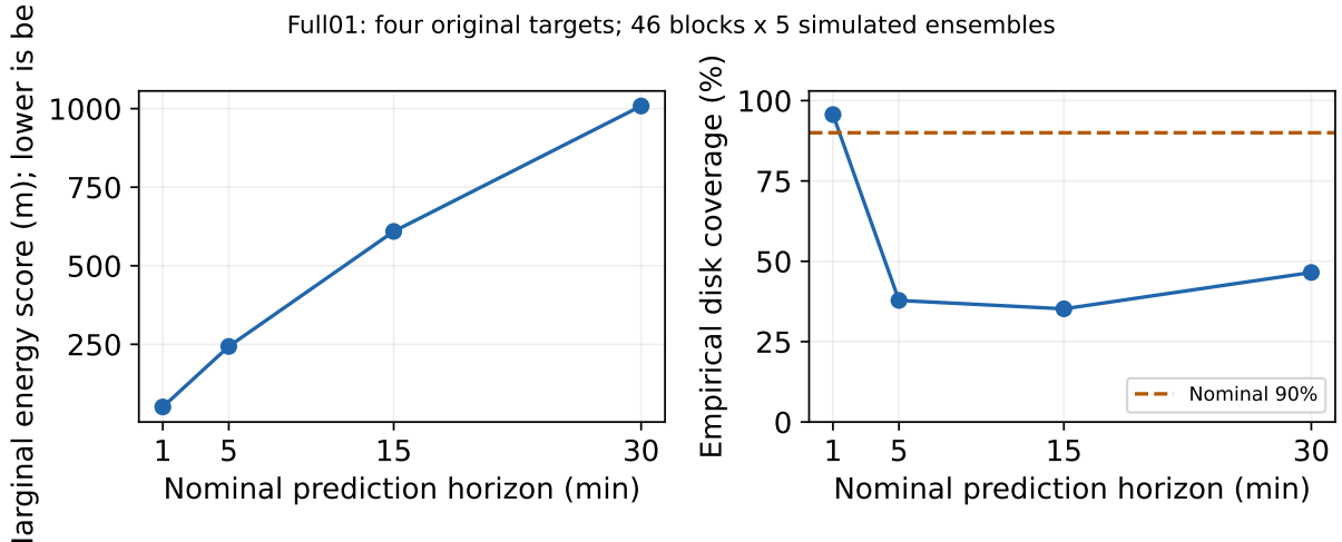
Figure 8: Full01’s actual aggregate saved scores and coverage at the four original targets. The dashed line is nominal 90% coverage; observed 30-minute coverage is only 46.52%. Lines guide the eye, not intermediate observations or a survival curve. These are distribution-level summaries, not trajectory/map overlays or independent 230-target measurements.
