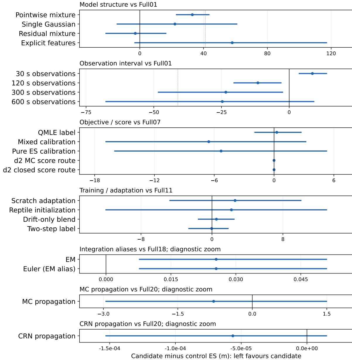
Figure 2: All 21 saved paired contrasts, with explicitly different horizontal scales. Points are recording-block means of candidate-minus-control ES; bars are saved within-family simultaneous 95% intervals. Each panel names its Full control; left of zero favours the candidate. Numerical panels are diagnostic zooms, not enlarged practical effects. Dotted \pm 41.10 -m boundaries appear only where within the axis range; they are outside the smaller panels. Neither zoom nor crossing a line qualifies a conclusion. The seven panels represent five method families: integration aliases, MC propagation and CRN propagation are three axes of the numerical family. Exact small differences and aliases remain in Table 24.
