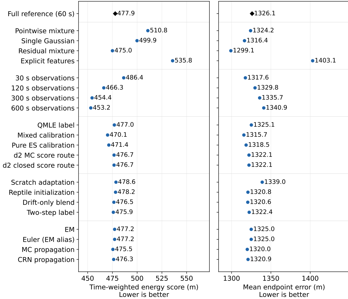
Figure 3: Full01 reference and all 21 candidates, with numeric labels for saved absolute ES and endpoint-error means in metres. Both dot axes are zoomed and lower is better; differences in dot position are not paired effect estimates. Observation variants follow increasing interval order. Six extra Full/replay roles are omitted only from this display and are retained separately, not averaged, in Table 51. Each row uses all 230 predictions; scoring routes and aliases are not independent algorithms. This is descriptive, not a global winner test.
