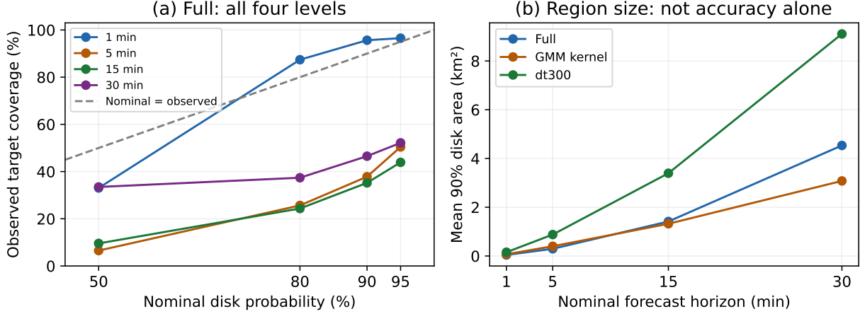
Figure 6: Saved calibration and region-size diagnostics, not new experiments. Left: Full’s observed coverage against nominal probability, separately for each horizon; the diagonal denotes nominal agreement. Right: mean 90% disk area for the three previously displayed models. Connecting lines only guide the eye between four measured levels or horizons; there is no intermediate target evaluation, simultaneous path coverage, or new statistical test.
