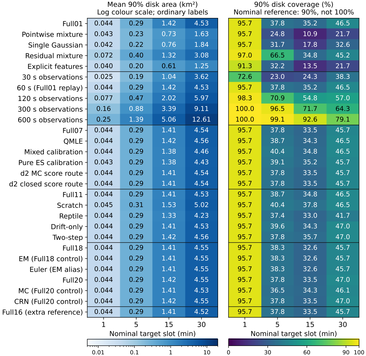
Figure 5: Complete 28-configuration region-size and coverage display at four original target slots. Left: mean nominal 90% disk area (km 2 ); colour uses a logarithmic scale to show both short- and long-horizon areas, while cell labels give ordinary areas. Right: empirical target containment (%), whose nominal reference is 90%, not 100%. Neither area nor coverage is a stand-alone quality ranking. Row order follows the declared method families, not observed performance; aliases and Full controls remain distinct. Each cell averages five seeds within each of 46 blocks and then equally over blocks. Descriptive means without new tests, prediction or recalibration; radii and exact values appear in Table 53 and the saved aggregate.
