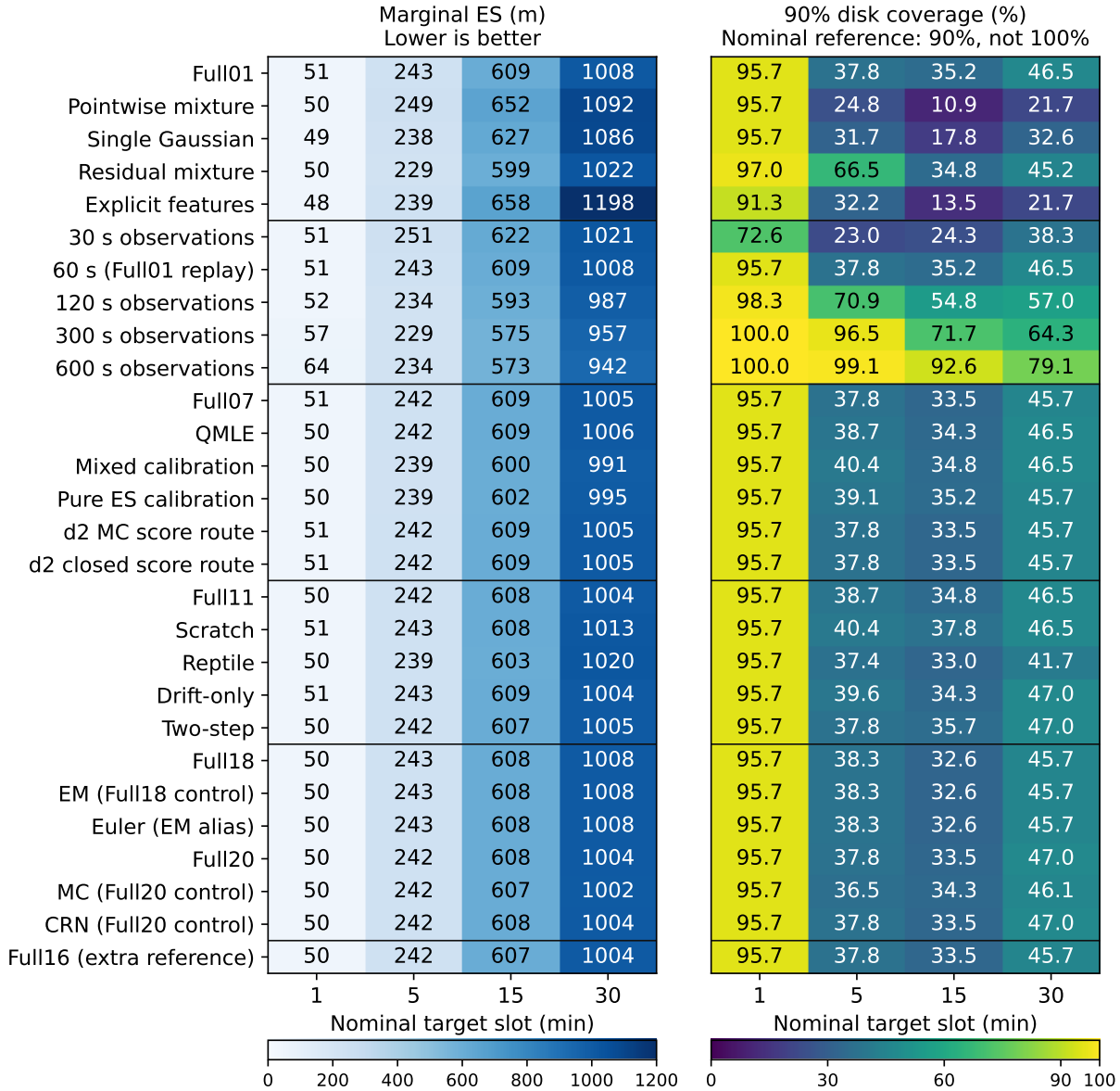
Figure 4: All 28 primary saved configurations at four nominal target slots; no intermediate-time prediction is added. Left: marginal ES (m), lower is better. Right: empirical nominal 90% disk coverage (%); 90% is the calibration reference, not 100%, and region sizes are not shown. Each cell averages the same 46 blocks and five seeds. ES is rounded to whole metres and coverage to one decimal for overview only; full-precision values and all roles remain in the saved projection and Table 52. Row order follows the declared families, not performance. Aliases and distinct Full controls are not pooled; similar rounded cells do not establish equivalence. Descriptive, not new per-horizon tests or final qualification.
