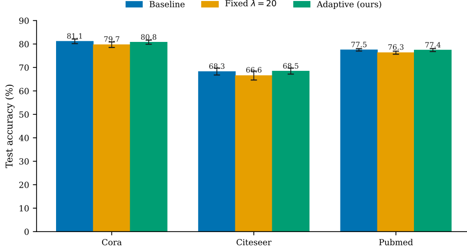
Fig. 1. Test accuracy of a 2-layer GAT on three citation networks under baseline training, fixed- \lambda ( \lambda = 20 ) diversity regularization, and feedback-controlled adaptive regularization (target 0.7, \eta = 0.05 ). Bars are means over 10 seeds; error bars are \pm 1 standard deviation over seeds; values above bars are means. The adaptive configuration stays within \pm 0.4 points of baseline on all three datasets; no fixed weight achieves both an effect on similarity and this level of accuracy (see Table 1).
