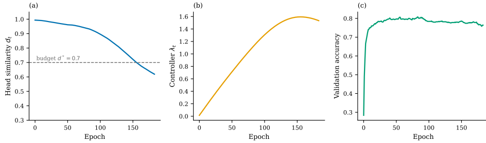
Fig. 2. Adaptive-controller dynamics on Cora, seed 3 (same-protocol run; see Sec. 5 for the provenance note): (a) head similarity d_t falls toward the 0.7 budget as (b) the integral controller raises \lambda ; (c) validation accuracy remains flat. The budget is enforced late in training, after the best checkpoint is selected.
