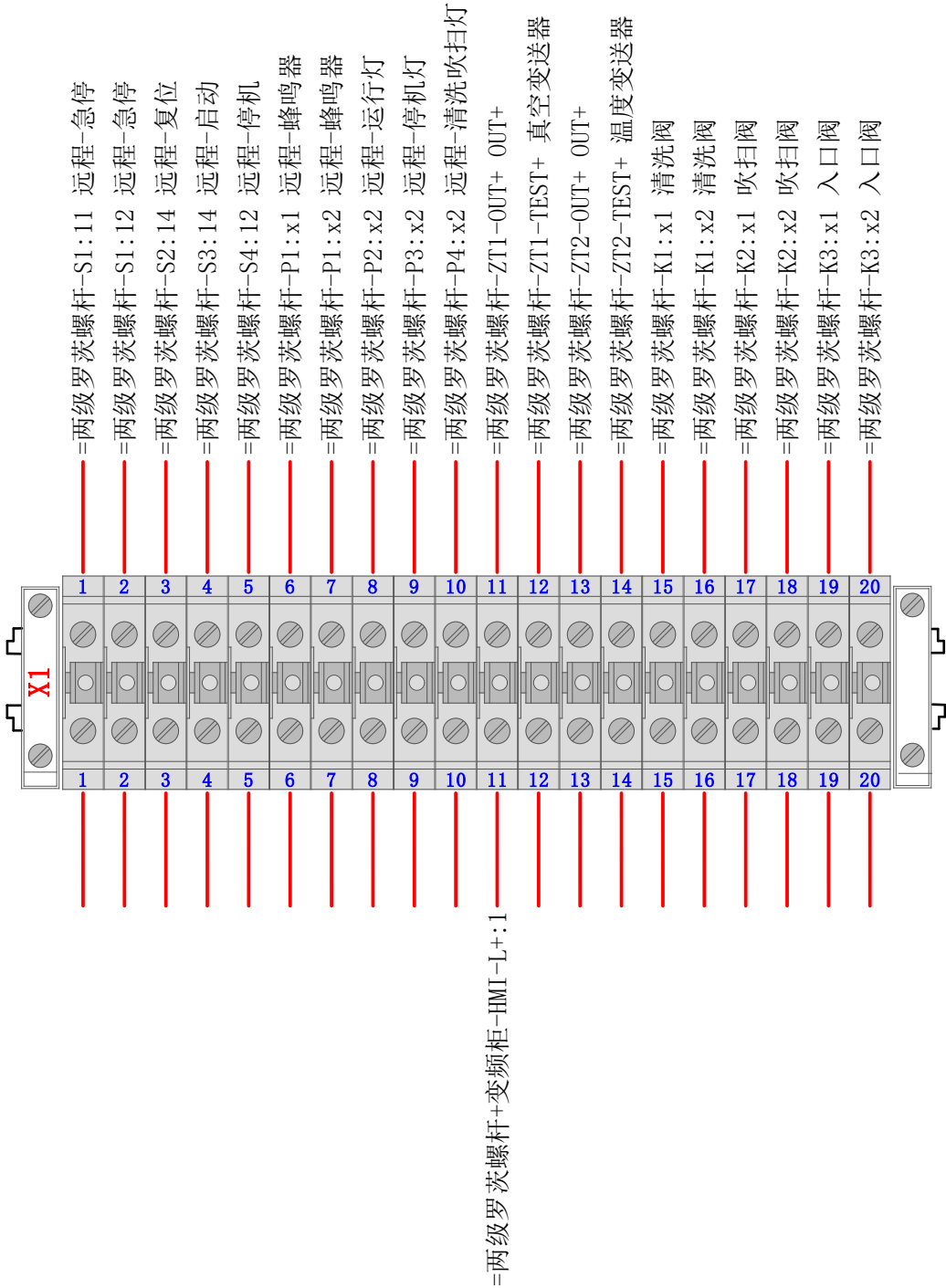
防爆操作柱X1~变频器柜X3
