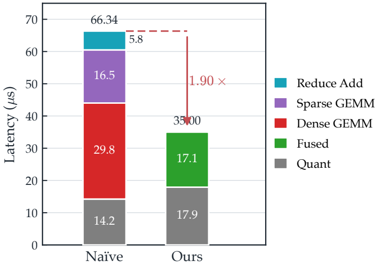
(a) Latency breakdown of W4A4 sparse-augmented GEMM
